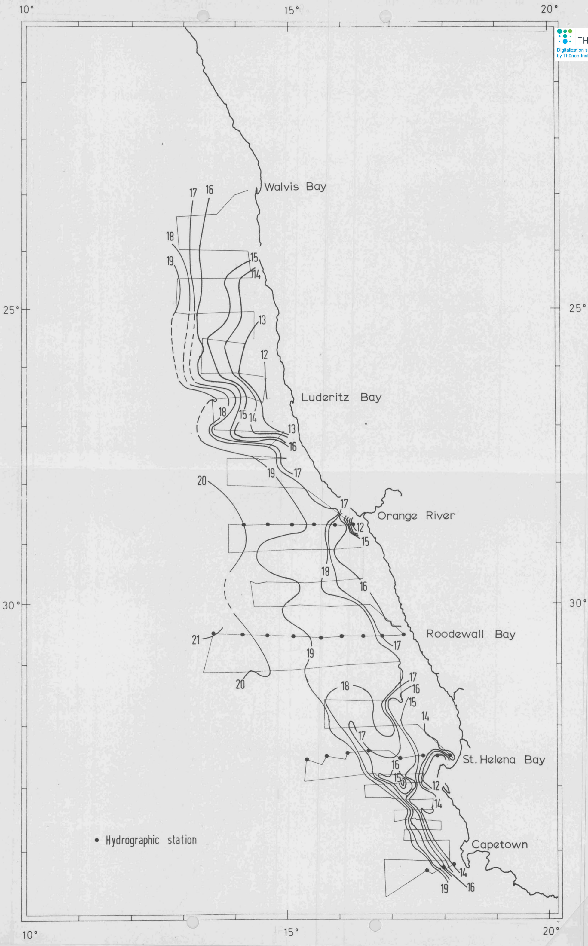
Figure 2 Surface temperature °C measured between 7-27 February 1966. Isotherms superimposed on ship's track.
